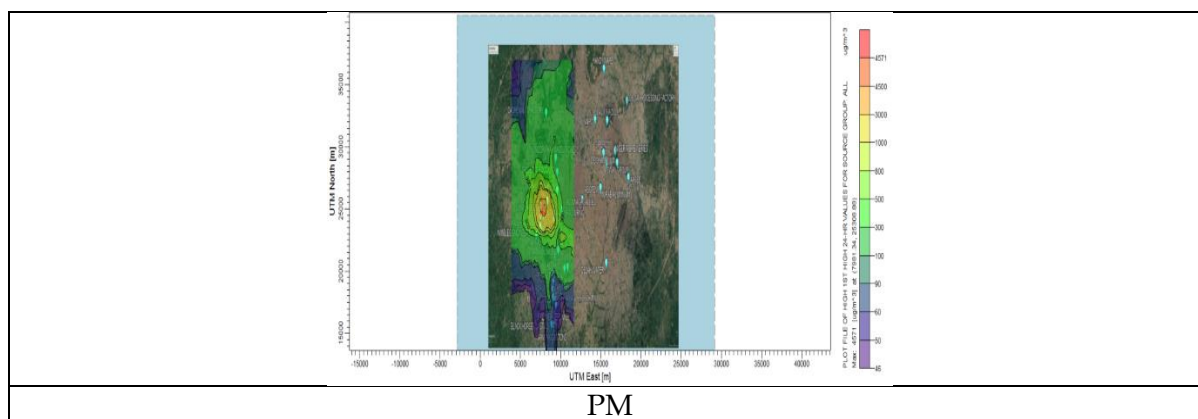
Fig 4: Predicted ground level concentration of Carbon monoxide (CO), Volatile Organic Compound (VOC), Particulate Matter (PM), Sulphur Oxide (SO x ) and Nitrogen Oxide (NO x ) respectively.
